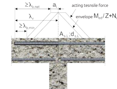
Figure 5 Anchoring of reinforcement to cover the line of acting tensile force.
