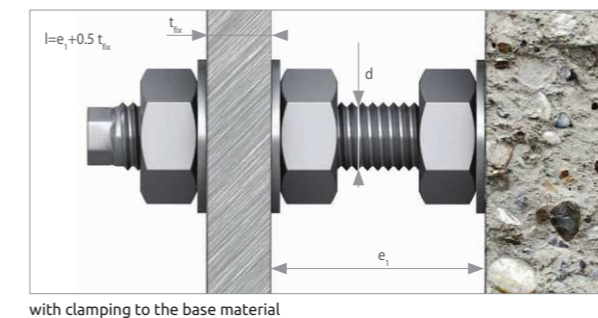
with clamping to the base material
