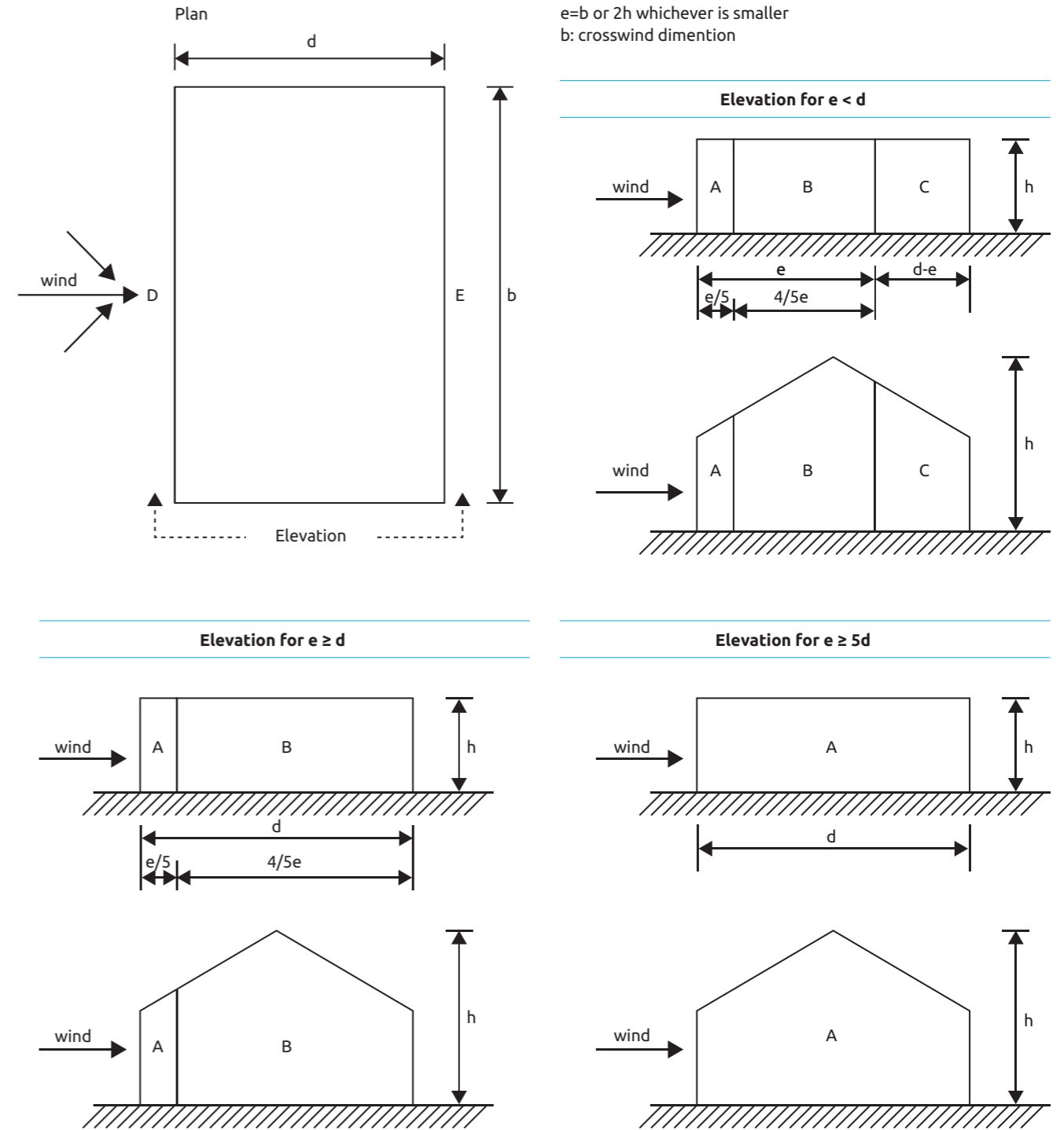
Figure 10.1 - Key for vertical walls
