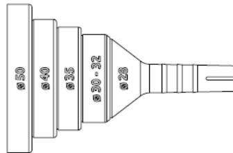
Hollow drill bit with vacuum cleaner
