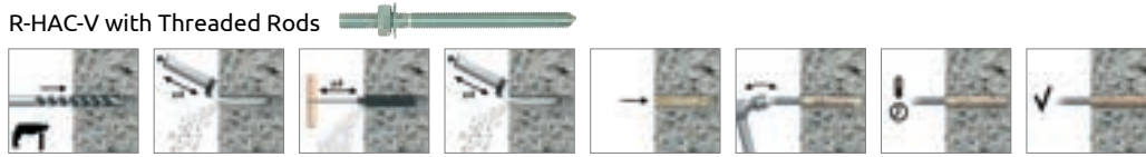
R-HAC-V with Rebar as an Anchor/ with Post-Installed Rebar
